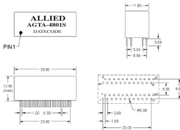
Dimensions: mm Unless otherwise specified, all tolerances are ±0.25
