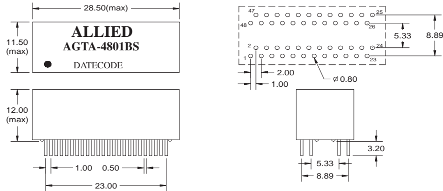
Dimensions: mm Unless otherwise specified, all tolerances are ±0.25
